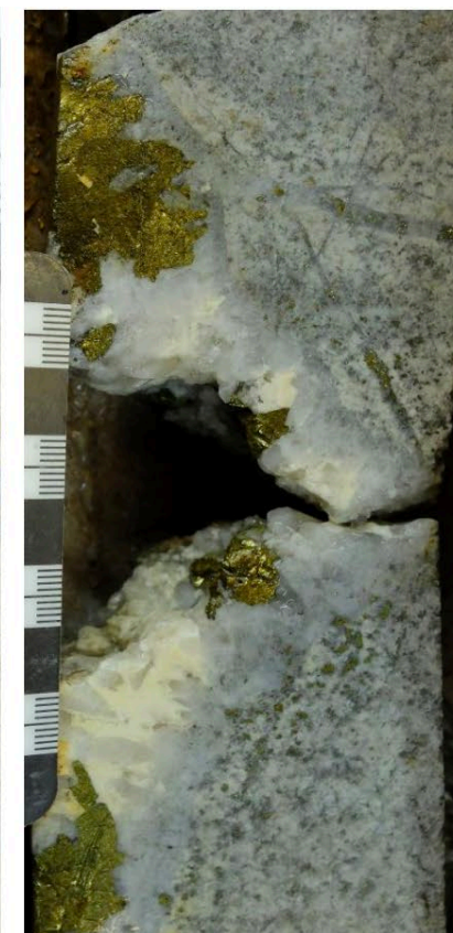
Breccia chalcopyrite- quartz cement
