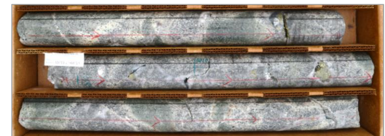
Core from mineralized breccia of drill hole FCD-23-024
